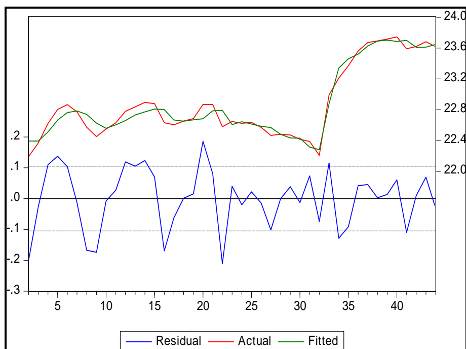
Figure 4. Residual Graph
